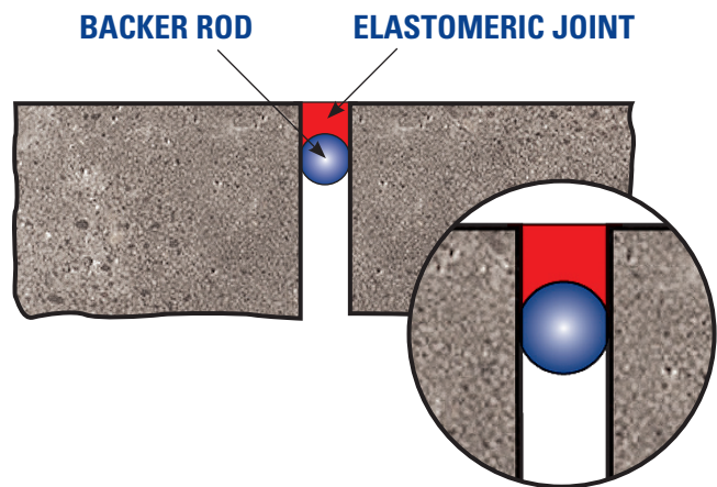
EXPANSION/ISOLATION JOINT
